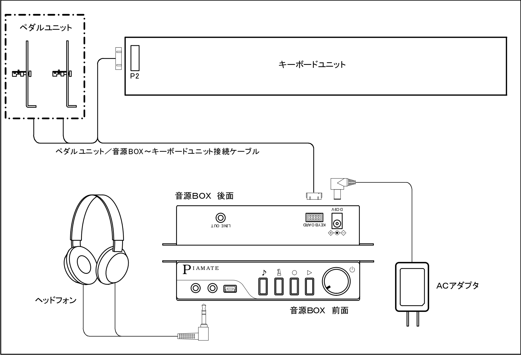
RB-900接続図
